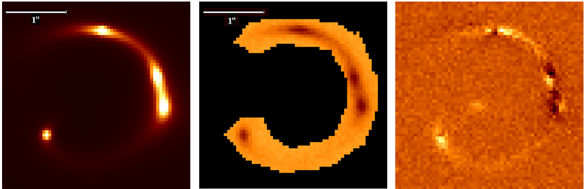
Figure 4. The left-hand panel shows an example of a simulated lens with noise and PSF (see Table 2 for details). The middle panel shows the reconstructed image of the lens inside the mask, using LENSED. The right-hand panel shows the unnormalized residual image of the data minus the model. The peak brightness of simulated lens and residuals are 1.30 and 0.37, respectively.
