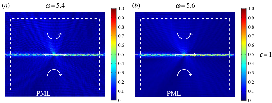
Figure 12. Displacement field in the homogeneous triangular lattice ( \varepsilon = 1 ) produced by a time-harmonic displacement, having a frequency (a) lower and (b) higher than the frequency at the Dirac point (figure 9f). In both cases, the absolute value of the spinner constant is |\alpha| = 0.9 . (Online version in colour.)
