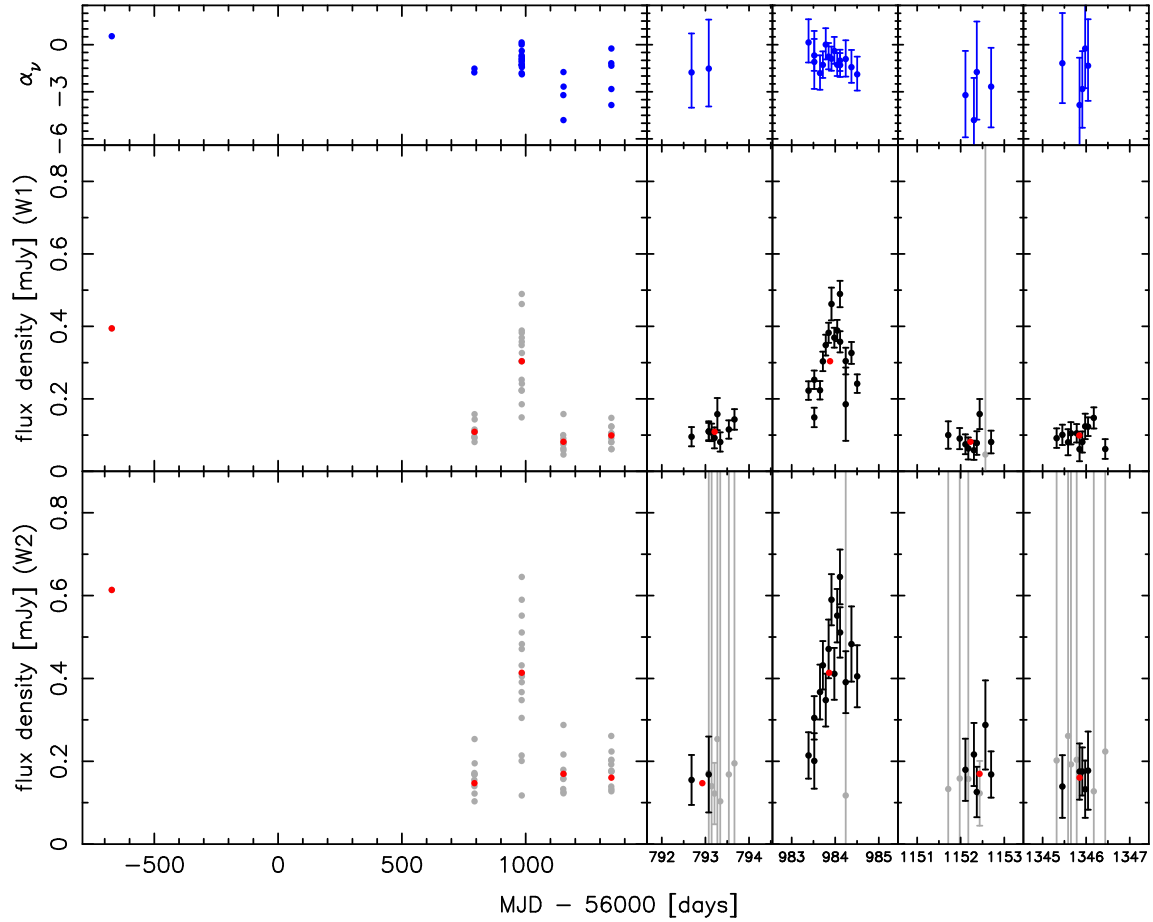
Fig. 6. (Top): Power-law indices calculated with the WISE 3.4\ \mu\text{m} and 4.6\ \mu\text{m} -band data as a function of time. (Middle), (Bottom): WISE light curves of J1100+4421 in the 3.4\ \mu\text{m} (W1) and 4.6\ \mu\text{m} (W2) -bands are shown in gray. The left panels are for the whole range of the WISE data while the other panels are magnified views of the four observing epochs of the NEOWISE Reactivation mission. In the four right panels, data points with < 0.5 mag errors are shown in black. Weighted averages of flux during each epoch is shown in red. The error bars are shown only in the magnified panels.
