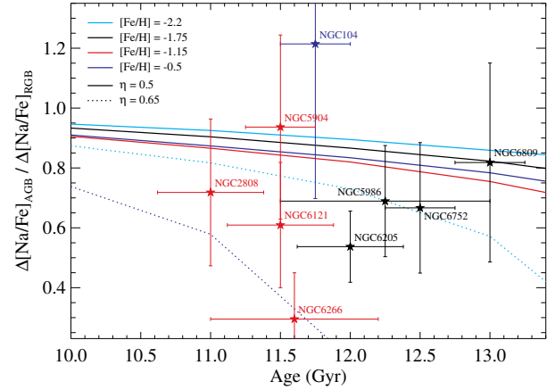
Fig. 11. Ratio of the [Na/Fe] spreads on the AGB and RGB as a function of GC age. Predictions of Charbonnel & Chantreau (2016) for the original FRMS scenario are shown for different values of metallicity (colors) and for two values of the \eta parameter adopted for Reimers mass loss along the RGB (0.5 and 0.65, solid and dotted lines respectively). The values derived in the present analysis are shown for the nine GCs (blue, red, and black stars, with the colors of the symbols indicating the theoretical track that has the closest [Fe/H] from that of each individual GC).
