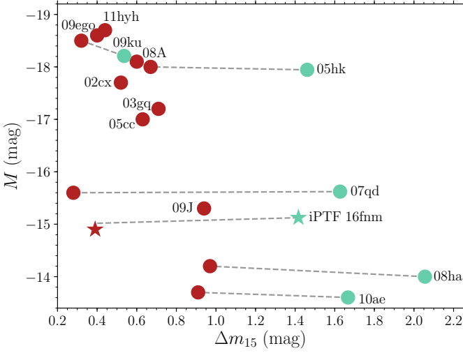
Figure 7. Absolute magnitude vs. \Delta m_{15} , both in the r' (shown in crimson) and g' -bands (teal) for 02cx-like SNe, adapted from White et al. (2015). The dashed grey lines connect SNe for which both r' and g' observations are available. Note that following White et al. (2015), we have not corrected M for host galaxy extinction, which is why SN 2010ae is fainter than SN 2008ha in this figure. In the r' band most 02cx-like SNe lie along a high-scatter sequence, though SN 2007qd and iPTF 16fnn are clear outliers. Similarly, g' -band observations of 02cx-like SNe also show weak evidence for a simple M - \Delta m_{15} relation.
