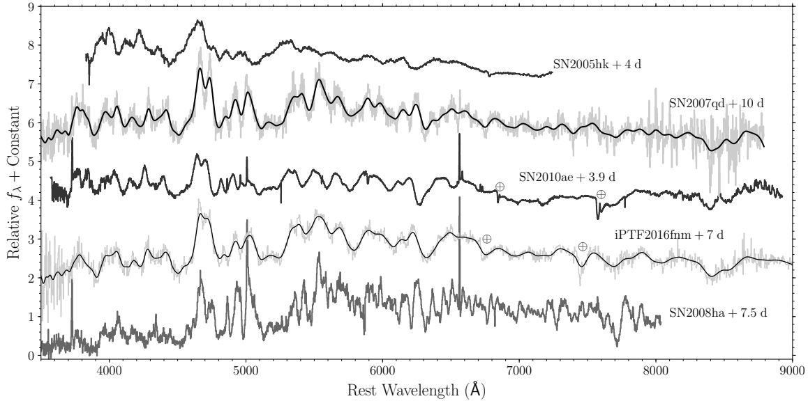
Figure 6. Spectral comparisons of iPTF 16fnn to other subluminal 02cx-like SNe. The spectra are labeled with their ages in the rest frame of the SN relative to B - or g' -band maximum. SN 2007qd and iPTF 16fnn are also shown following convolution with a FWHM = 2,500 km s -1 gaussian kernel. From top to bottom, the spectra are SN 2005hk (Phillips et al. 2007), SN 2007qd (McClelland et al. 2010), SN 2010ae (Stritzinger et al. 2014), iPTF 16fnn, and SN 2008ha (Foley et al. 2009). SN 2005hk is a prototypical 02cx-like SN, while SNe 2007qd and 2010ae, like iPTF 16fnn, were fainter at the time of maximum brightness with lower expansion velocities. SN 2008ha is the faintest member of the 02cx-like class.
