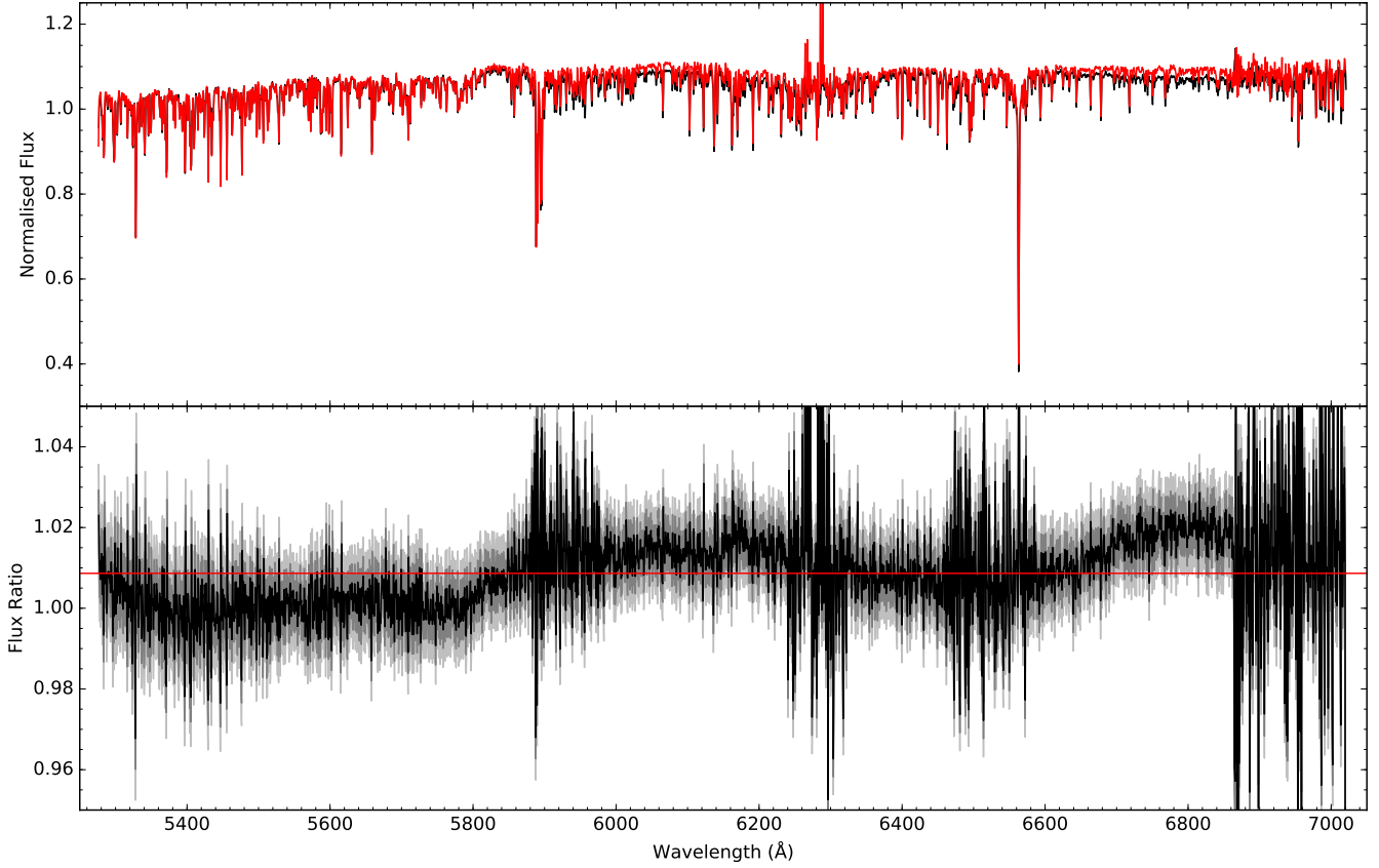
Figure 11. Top: Comparison of the R7000 integrated spectra of NGC 2808 from 2015-01-31 (black) and from 2015-07-09 (red). This is a relative comparison as both observations have been normalised such that their mean flux between 5300 Å to 5500 Å is unity. The 2015-01-31 spectrum has a S/N of 744 \text{ Å}^{-1} while the 2015-07-09 spectrum has a S/N of 389 \text{ Å}^{-1} . These S/N are based on the uncertainties provided by the PyWiFES pipeline. The spectra have been shifted to the rest frame. Bottom: Ratio of the two nights observations in black. The dark grey and light grey regions show the one and two sigma uncertainties in the ratio. We note that the regions of greatest variance - 5880 to 5980 Å, 6270 to 6330 Å, 6460 to 6580 Å and redwards of 6860 Å - lie in wavelength regions affected by telluric lines.
