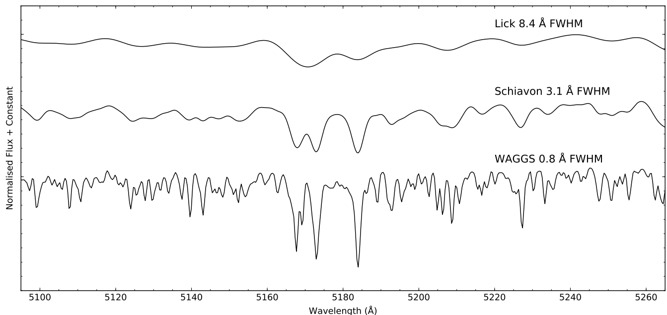
Figure 4. WAGGS spectral resolution compared to previous work. Our spectrum of NGC 104 around Mg_b is plotted at its original spectral resolution ( R = 6800 , 0.8 \text{ Å FWHM} , bottom), smoothed to the spectral resolution of Schiavon et al. (2005) library of GC spectra ( R = 1700 , 3.1 \text{ Å FWHM} , middle) and of the Lick index system (Worthey et al. 1994, R = 600 , 8.4 \text{ Å FWHM} , top). The smoothed spectra have been offset in flux for legibility. This NGC 104 spectrum has a S/N of 689 \text{ Å}^{-1} . Our spectra have four times higher spectral resolution compared to the spectra of Schiavon et al. (2005) and eleven times the spectral resolution of the Lick system. This high resolution allows us to study much weaker spectral lines. Note that the apparently smooth pseudo-continuum at low resolution is made up of numerous weak absorption lines.
