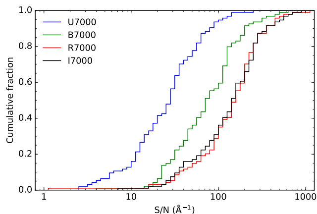
Figure 5. Cumulative S/N per \text{Å} distributions of the integrated spectra for each of the gratings. In general the S/N of the U7000 spectra is lower than the B7000 spectra while the R7000 and I7000 are higher.
