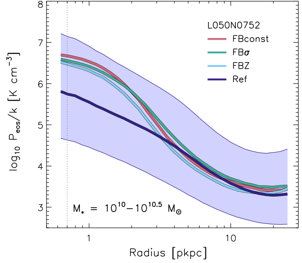
Figure 8. The birth pressure of star particles, as a function of galactocentric radius, for galaxies with stellar mass 10 < \log_{10} M_{\star}/M_{\odot} < 10.5 at z = 0.1 . Solid curves denote the binned median, and the blue shaded region corresponds to the 1\sigma scatter about the median of Ref. The dotted vertical line shows the gravitational softening scale. The highest pressures correspond to stars formed in galactic centres, so numerically inefficient feedback in the FBconst, FB \sigma and FBZ models leads to the formation of unrealistically massive central spheroids. Conversely, the suppression of high birth densities in Ref yields effective radii that are consistent with observations. The convergence of the birth pressure profiles for r \gtrsim 4 \text{ pkpc} indicates that differences in the heating rate of gas (i.e. f_{\text{th}} ) between the models are confined to galactic centres.
