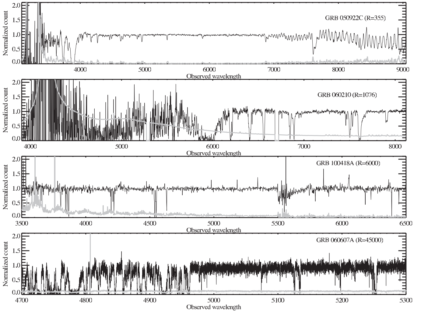
Figure 1. Comparison between four different GRB spectra obtained with different spectrographs and different resolving power. From top to bottom: GRB 050922C observed with ALFOSC; GRB 060210 observed with Gemini/GMOS; GRB 100418A observed with the UV arm of VLT/X-Shooter; section of GRB 060607A observed with VLT/UVES. In all panels, the gray curve represent the associated 1\sigma error spectrum.
