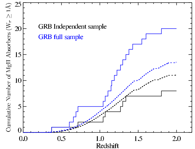
Figure 7. Cumulative distribution of strong Mg II absorbers along GRB sight lines for Sample I and Sample F (black and blue solid curves, respectively). These are compared to the predicted incidence based on measurement along QSO lines of sight (dashed curves). The independent Sample I actually shows fewer absorbers than expected while a modest excess remains in Sample F. Neither result corresponds to a statistically significant difference from the QSO results.
