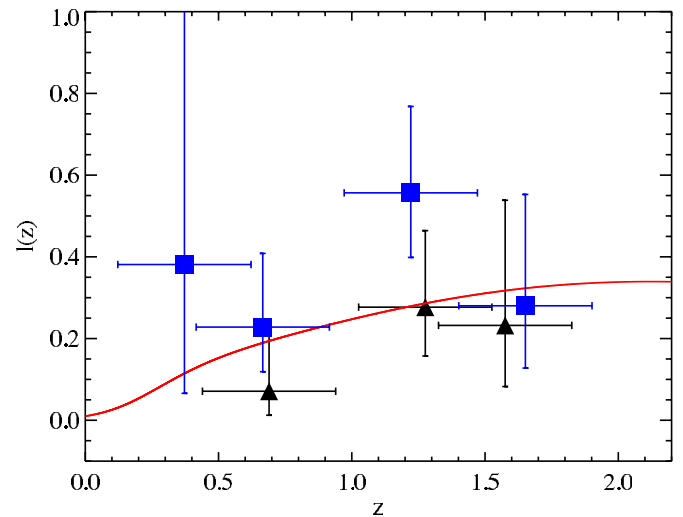
Figure 6. \ell(z) evolution of intervening Mg II absorbers ( W_{2796} \geq 1 \text{ \AA} ) for our sample of GRB sight lines: triangles and square symbols refer to the Sample I and Sample F, respectively. The red curve shows the evolution of the Mg II incidence along quasar sight lines as recently computed by Zhu & Menard (2012). We derive an average \ell(z) = 0.20 for Sample I, in agreement with the prediction, while \ell(z) = 0.36 for Sample F, indicating a slight overabundance of absorbers compared to the QSOs.
