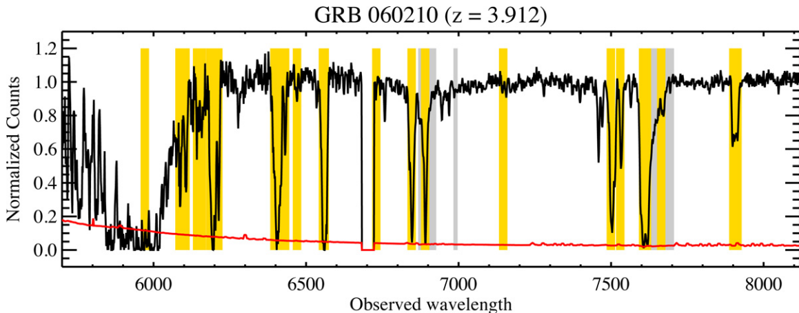
Figure 2. GRB 060210 Gemini spectrum. This example shows our excluded regions for the purpose of estimating the survey path for intervening \text{Mg II} absorption taking into account the host absorption lines (in gold, from the tabulation of Christensen et al. 2011) as well as telluric lines (in gray). The red curve is the 1\sigma spectrum associated with the data.
