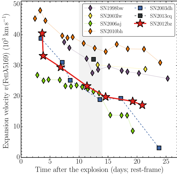
Fig. 5. Evolution of the expansion velocities measured from FeII \lambda 5169 for SN 2012bz and six GRB-SNe of low (diamonds) and high-luminosity GRBs (boxes) with good spectroscopic data. Measurements were performed on our data as well as on the spectra of Patat et al. (2001), Hjorth et al. (2003), Malesani et al. (2004), Pian et al. (2006), and Bufano et al. (2012). The value of SN 2013cq was taken from Xu et al. (2013). The grey-shaded area displays the interval of observed GRB-SN peak times.
