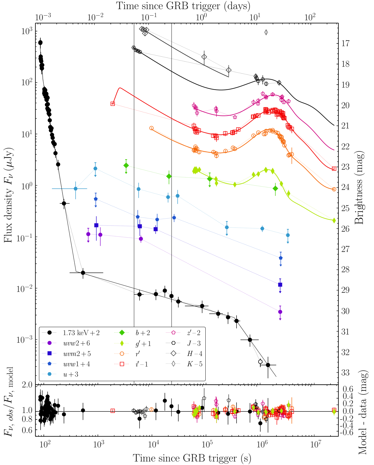
Fig. 2. X-ray, optical and NIR light curves of the transient that followed GRB 120422A. Arrows indicate 3\sigma upper limits. The UVOT u -band upper limits are very shallow and not displayed. Data in the g'r'i'z' bands were modelled with a rescaled SN 1998bw template at z = 0.283 , which was superposed on a power-law (where the slope was identical in all bands) using the formalism in Zeh et al. (2004). The best-fit model parameters are shown in Table 3. Model light curves in bluer or redder filters are not shown, since they would require extrapolation of the spectral range of the SN1998bw template. Fit residuals are displayed in the bottom panel. The XMM-Newton observation was carried out at 980 ks (open dot). The shifts (in magnitude) of the different bands are given in the legend. To convert the X-ray light curve to flux density, we assumed a spectral slope of \beta = 0.9 and no spectral evolution (for details on the SED modelling see Sect. 3.2.3). Both assumptions have no implications on our analysis. The XMM-Newton data point was discarded from the light curve fit because of uncertainties in the cross-calibration between Swift /XRT and XMM-Newton . The vertical lines indicate the epochs of the X-ray-to-NIR SEDs presented in Sect. 3.2.3. Error bars can in some cases be smaller than the marker size.
