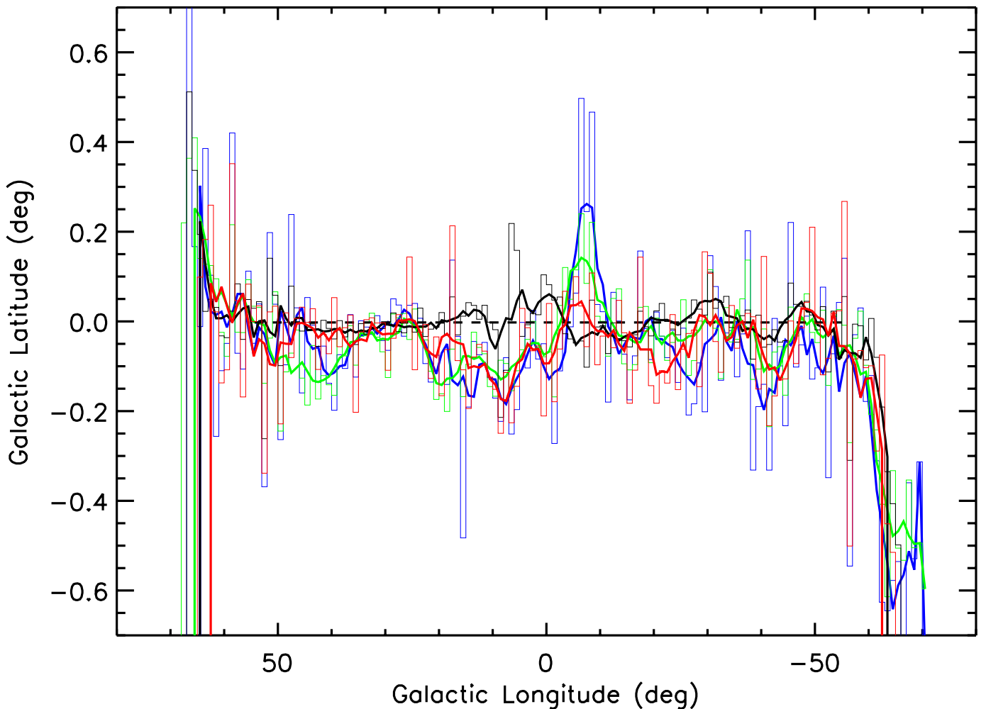
Fig. 4: Histograms representing the distribution of the median Galactic latitude of the Hi-GAL sources detected at 70\,\mu\text{m} (blue line) and at 250\,\mu\text{m} (green line), each with counterparts in at least two adjacent bands. The histograms are computed in 1^\circ longitude bins, together with the analogous distribution of entire sample of MIPS GAL 24\,\mu\text{m} sources (black line); the distribution of the subsample of MIPS GAL 24\,\mu\text{m} sources selected by Robitaille et al. (2008) using color criteria targeted toward YSOs is shown with the red line. The thick coloured lines show the result of a 5^\circ -wide running boxcar smooth. The horizontal dashed black line reports the median latitude of all MIPS GAL 24\,\mu\text{m} sources that essentially coincides with the nominal b=0^\circ midplane.
