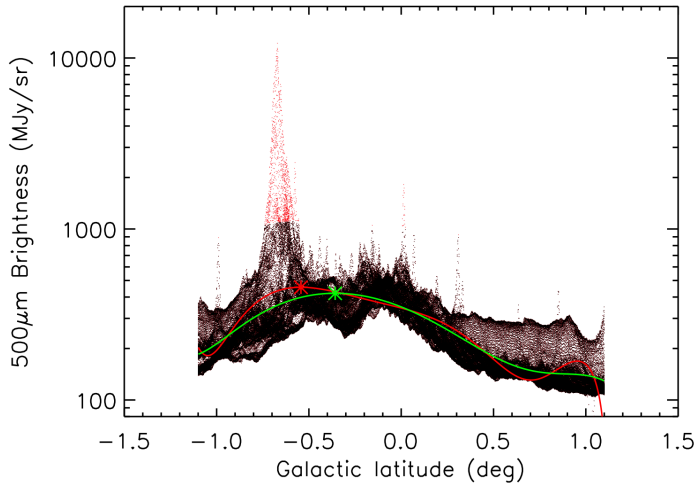
Fig. 2: 500- \mu m brightness values (all the points) as a function of Galactic latitude in the longitude interval 14.5 \leq l \leq 15.5 from the map in fig. 1b (this longitude range contains M16, which is clearly visible as the large bump at b \sim -0.7 ). The red thick line is the 7 th -order polynomial fit to all points, and the red points are those that are clipped away as they lie above 3 times the r.m.s. of the residuals (after subtracting the fit). The green thick line is the 5 th -order polynomial fit to all points that survived this clipping (all the black points). The thick crosses mark the positions of the maxima of each respective fit.
