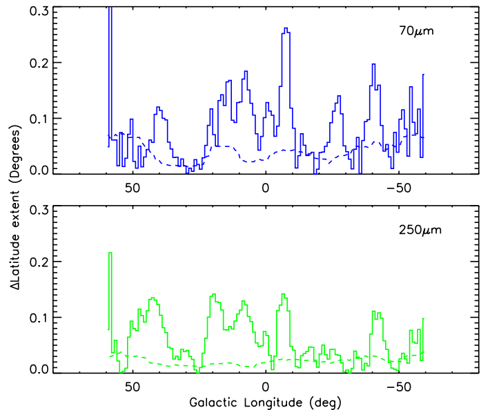
Fig. 5: Full-line histograms representing, as a function of longitude, the absolute value of the smoothed median source latitude (the thick lines of fig. 4), and the running standard deviation (dashed lines) of the residuals between the median latitude and its smoothed function (i.e., the difference between the thin and thick lines in fig. 4), computed using a boxcar of 10 degrees. The upper panel shows the result for the 70- \mu\text{m} sources in blue, and the lower panel shows the 250- \mu\text{m} sources in green. Note that we are using only those Hi-GAL sources with a counterpart in at least 3 adjacent bands.
