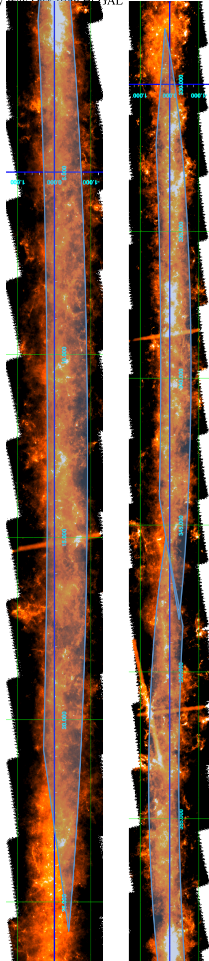
Fig. 1: b ) As fig. 1a, but for the longitude ranges 0^\circ \leq l \leq 27^\circ (upper panel) and 327^\circ \leq 360^\circ (lower panel), encompassing the range spanned by the Galactic Bar.
