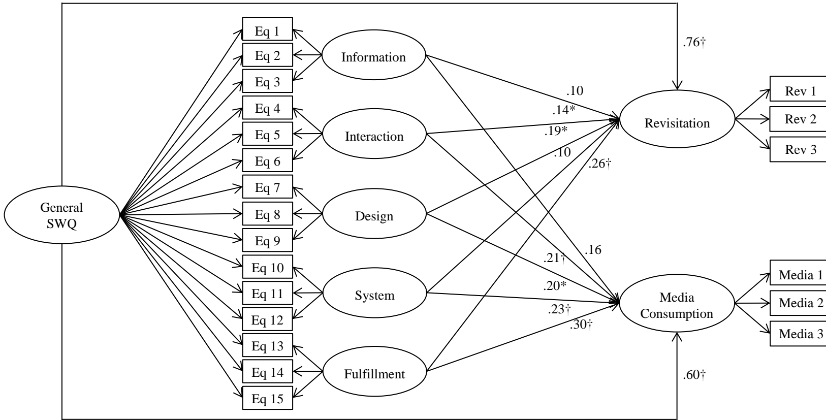
Fig. 3. Hypothesized simultaneous equations model of Sports Website Quality (SWQ) ( \chi^2=300.36 , df=162 , \chi^2/df=1.85 ; CFI=.97, TLI=.962, RMSEA=.06, SRMR=.05). * p<.05 . † p<.001 .
