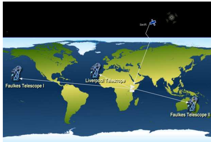
Fig. 2. The locations of the 2-m robotic Liverpool Telescope and its clones the Faulkes telescopes. GRB triggers from satellites drive prompt automatic follow up.
