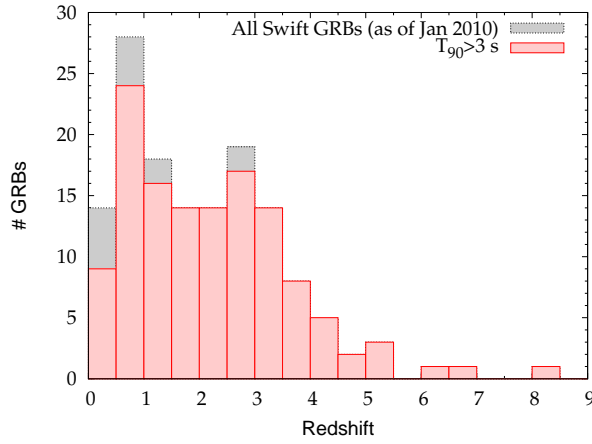
Fig. 1. Redshift distribution of Swift GRBs detected to-date.
