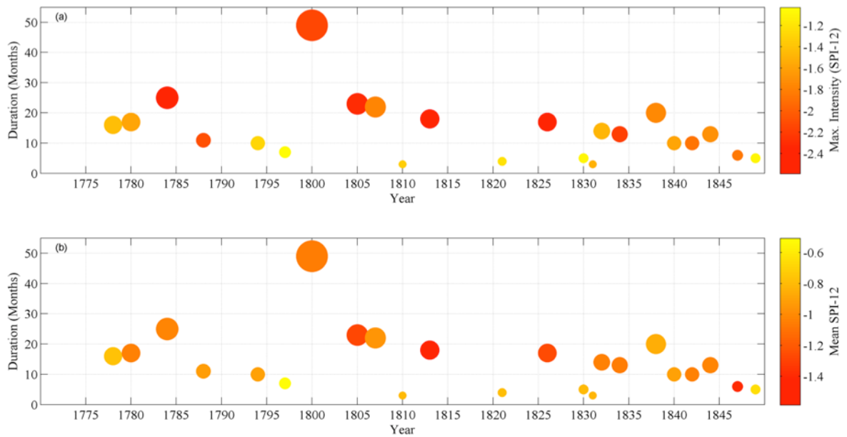
Figure 8. Drought duration plotted against a). maximum intensity and b). mean SPI-12 for each of the 23 droughts identified in the Island of Ireland extended (IoIext) series 1765-1849. Circle size denotes duration (months) while the colour ramp indicates intensity and mean SPI-12 respectively.
