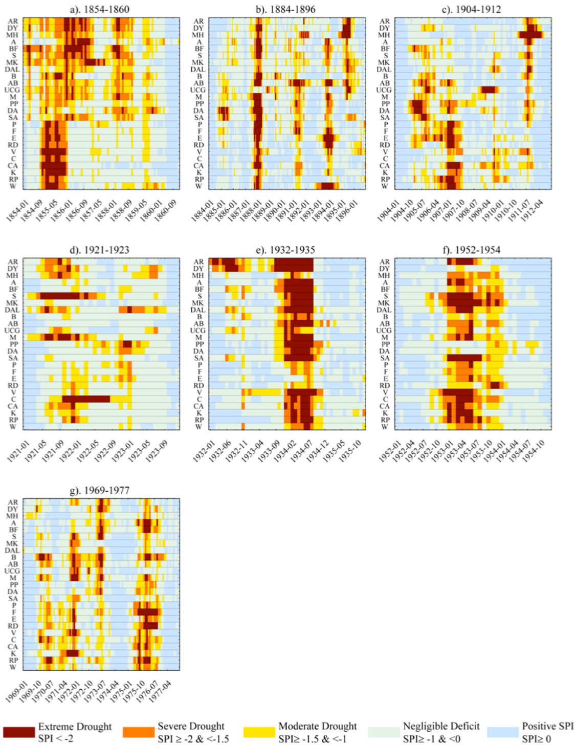
Figure 6. Drought signatures showing SPI-12 values for all stations in the Island of Ireland Precipitation (IIP) network for the 7 drought periods identified with island wide impact. Negative SPI-12 values are colour coded according to severity thresholds to highlight periods of moderate to extreme drought conditions.
