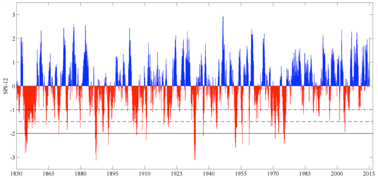
Figure 2. SPI-12 series for the Island of Ireland (IoI) series 1850-2015. Dotted horizontal line is the threshold for drought start (-1.0), the dashed horizontal line is the threshold for severe drought (-1.5) and solid horizontal line is the threshold for extreme drought (-2.0).
