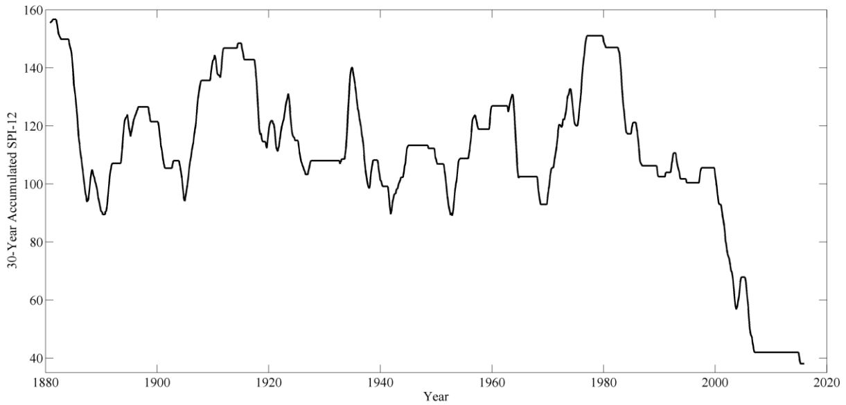
Figure 4. 30-year accumulated SPI-12 values for identified drought events in the Island of Ireland (IoI) series. Note that the end year of each 30-year accumulation period has been used to define the x-coordinate plotting position, and that the accumulated SPI values have been multiplied by -1 so that lower values indicate a deficit of dry conditions.
