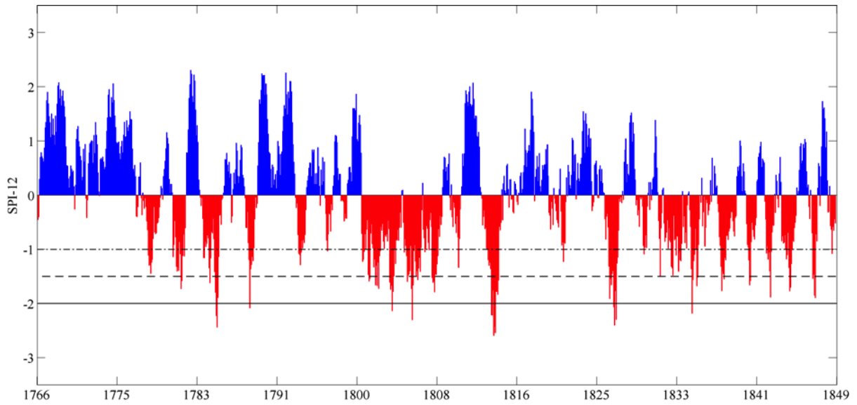
Figure 7. SPI-12 series for the Island of Ireland extended (IoIext) series 1765-1849. Dotted horizontal line is the threshold for drought start (-1.0), the dashed horizontal line is the threshold for severe drought (-1.5) and solid horizontal line is the threshold for extreme drought (-2.0).
