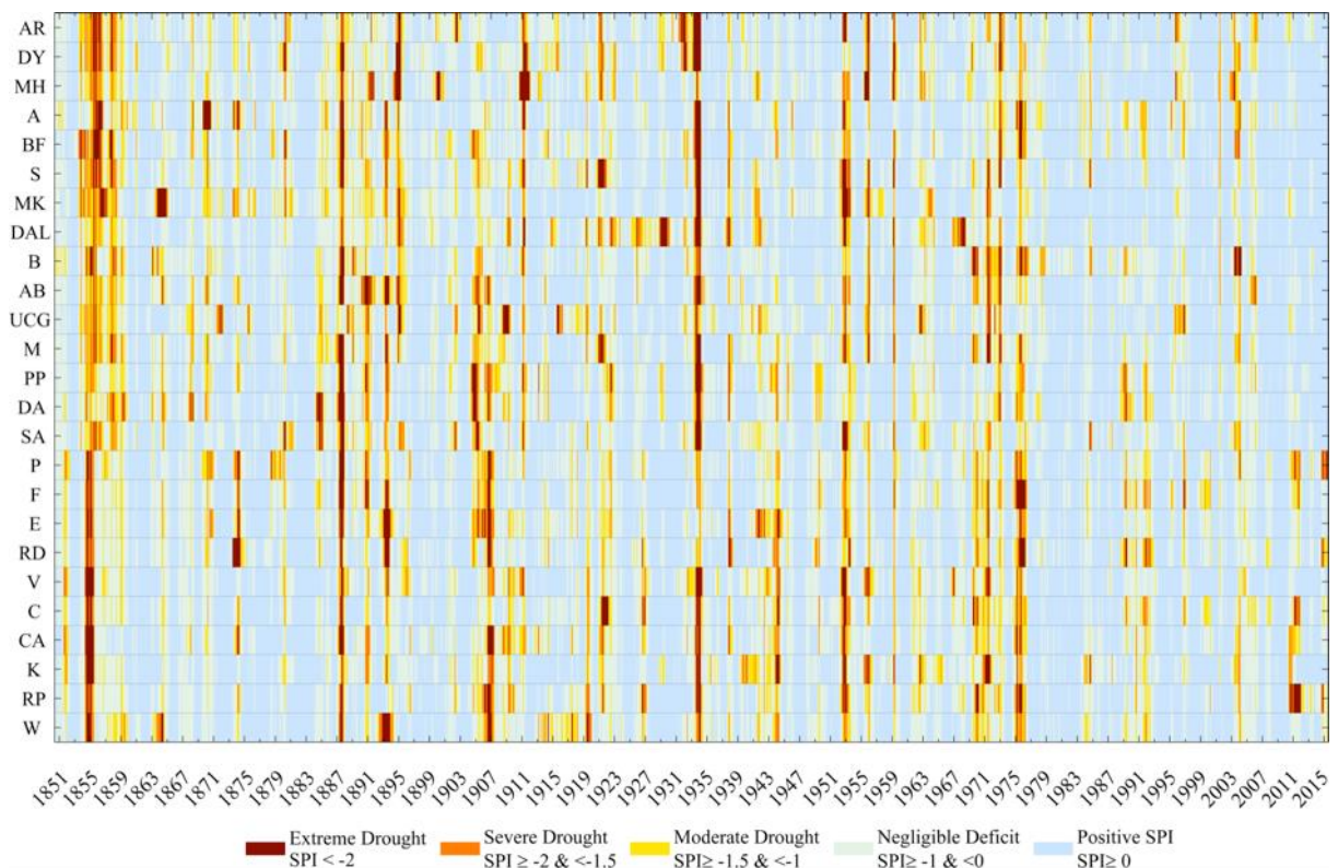
Figure 5. SPI-12 values for all 25 stations in the Island of Ireland Precipitation (IIP) network. Negative SPI-12 values are colour coded according to severity thresholds to highlight periods of moderate to extreme drought conditions.
