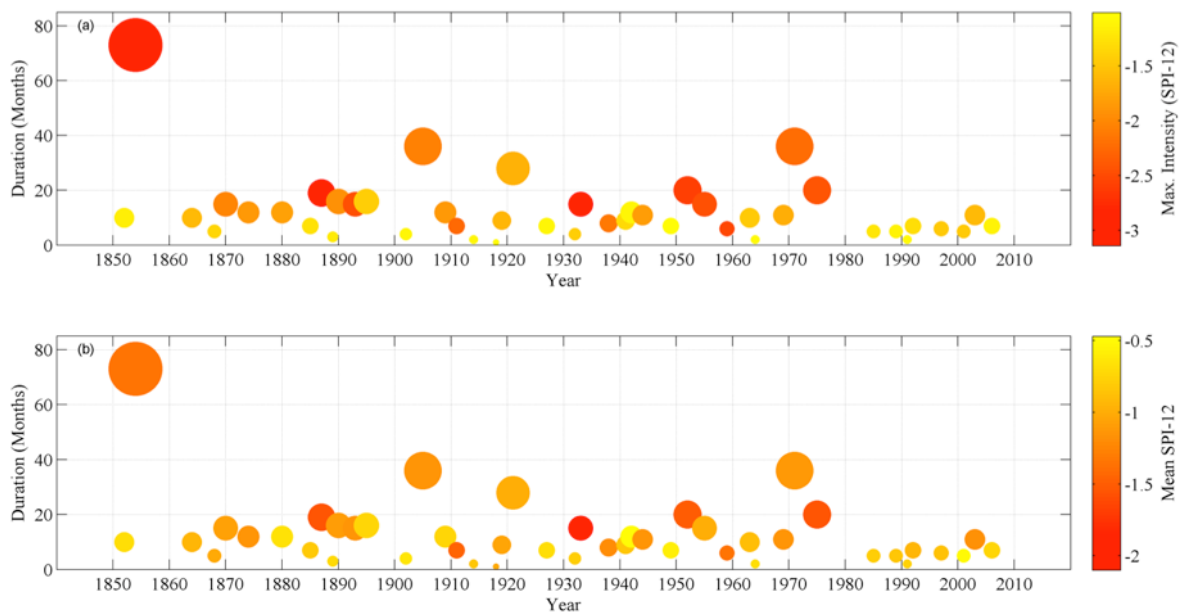
Figure 3. Drought duration plotted against a). maximum intensity and b). mean SPI-12 for each of the 45 droughts identified in the Island of Ireland (IoI) series 1850-2015. Circle size denotes duration (months) while the colour ramp indicates intensity and mean SPI-12 respectively.
