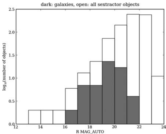
Figure 2. Number counts for the galaxies and SECTRATOR-selected objects. The grey histogram shows the number counts for galaxies with redshifts and the open histogram for all objects. The object catalogue list appears complete to R = 21.5 . The galaxy completeness drops significantly at R > 20.5 .
