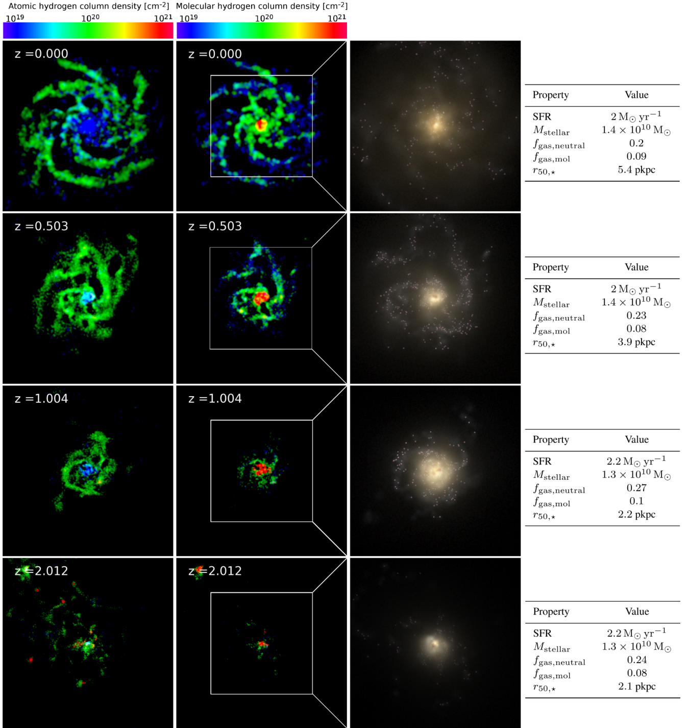
Figure 6. Visualization of four galaxies in EAGLE (at redshifts z = 0, 0.5, 1 and 2 ) which were chosen to have M_{\text{stellar}} \approx 10^{10} \text{ M}_{\odot} , \text{SFR} \approx 2 \text{ M}_{\odot} \text{ yr}^{-1} and f_{\text{gas, neutral}} \approx 0.25 . The redshift of each galaxy is shown in the H I and H 2 maps. The H I and H 2 maps are coloured by column density, according to the colour bars at the top, with column densities in units of \text{cm}^{-2} . The right-hand panels show SDSS gri images, which were constructed using the radiative transfer code SKIRT (Baes et al. 2011, see Trayford et al. in preparation for details). Particles are smoothed by 1 ckpc in the N_{\text{H}_2} and N_{\text{H}_1} maps. H I and H 2 maps have a size of 100 \times 100 \text{ pkpc}^2 , while the gri images are of 60 \times 60 \text{ pkpc}^2 (scale that is shown in the middle panels as a white square frame). At the right of every row we show the integrated values of the stellar mass, SFR, neutral gas fraction, molecular gas fraction and the projected half-stellar mass radius. Masses and SFR were calculated in spherical apertures of 30 pkpc, while the radius is calculated using a 2D circular aperture of 30 pkpc (averaged over three orthogonal projections).
