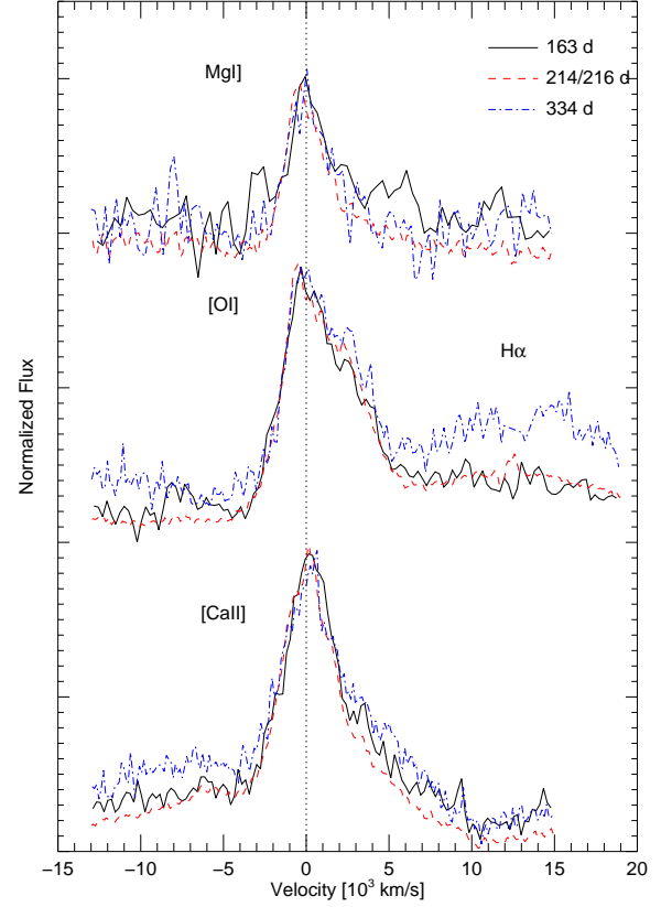
Figure 11. Nebular emission line profiles of SN 2011hs from 163 days, 214/216 days and 334 days spectra.
