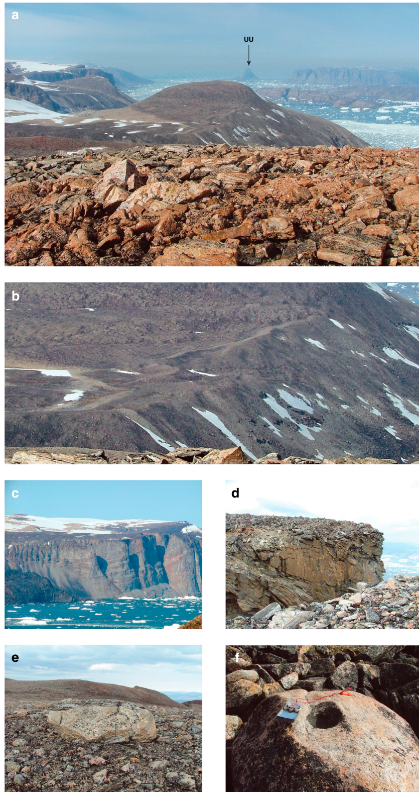
Figure 6. (a) The upper surface of the northern edge of the Nuussuaq Peninsula looking west towards Uummanaq. Note the angular blockfield terrain and undulating topography. (b) Along the edge of the plateau, push moraines can be seen overtopping the plateau edge (~750–800 m asl). (c) Below ~750 m asl, the wall of the fjord are clearly glacially scoured. (d) The blockfield on the plateau is derived from ~2 m of in situ shattered bedrock (field of view ~40 m wide), though erratics up to 2 m in diameter can be found on the blockfield between 750 and 1200 m asl (e), some of which exhibit weathering pits (f).
