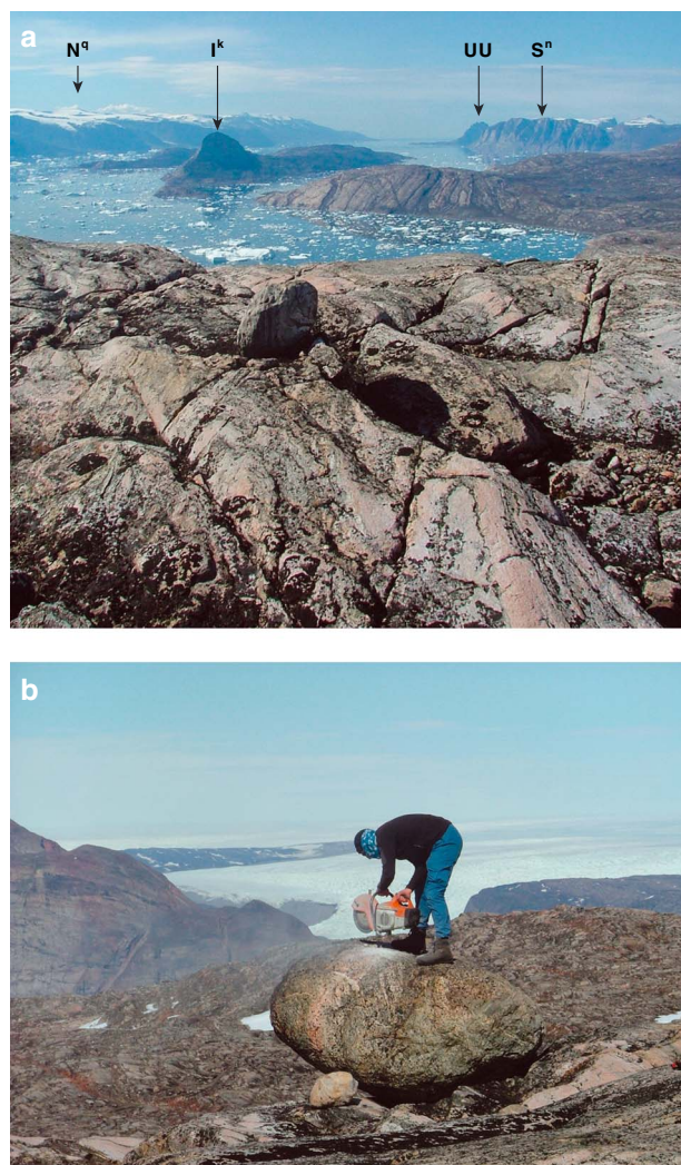
Figure 5. (a) Areally scoured terrain on Drygalski Halvø (960 m asl) looking west across Ikerasak (Ik) and the Nuussuaq Peninsula (Nq), Storøen (Sn), and Uummannaq (UU). (b) Perched sub-glacial erratic situated on areally scoured terrain on Drygalski Halvø (DH) (e.g., Sample IKE 1; 11.4 ka; Table 2).
