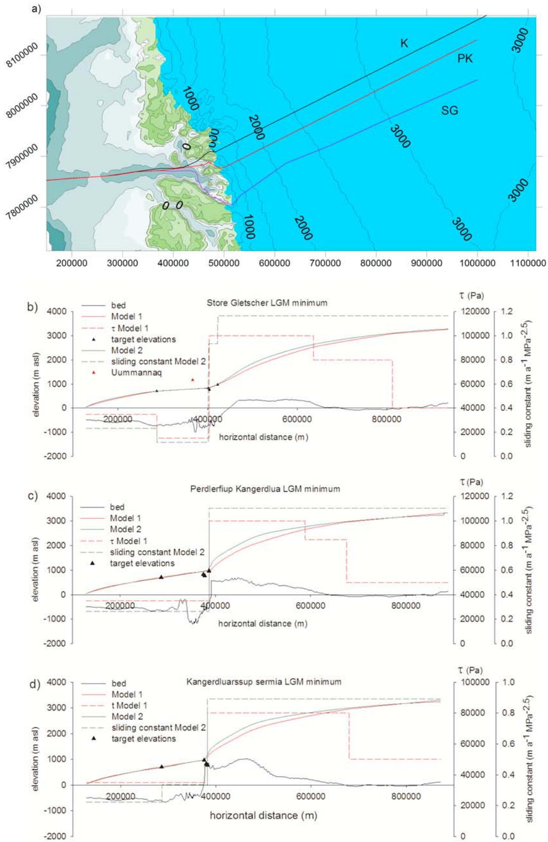
Figure 10. (a) Location of ice sheet surface profiles. SG = Store Gletscher; PK = Perdlerfiup Kangerdlua; K = Kangerdluagssup sermia. (b) Minimum LGM surface profile for Store Gletscher. (c) Minimum LGM surface profile for Perdlerfiup Kangerdlua. (d) Minimum LGM surface profile Kangerdluagssup sermia.
