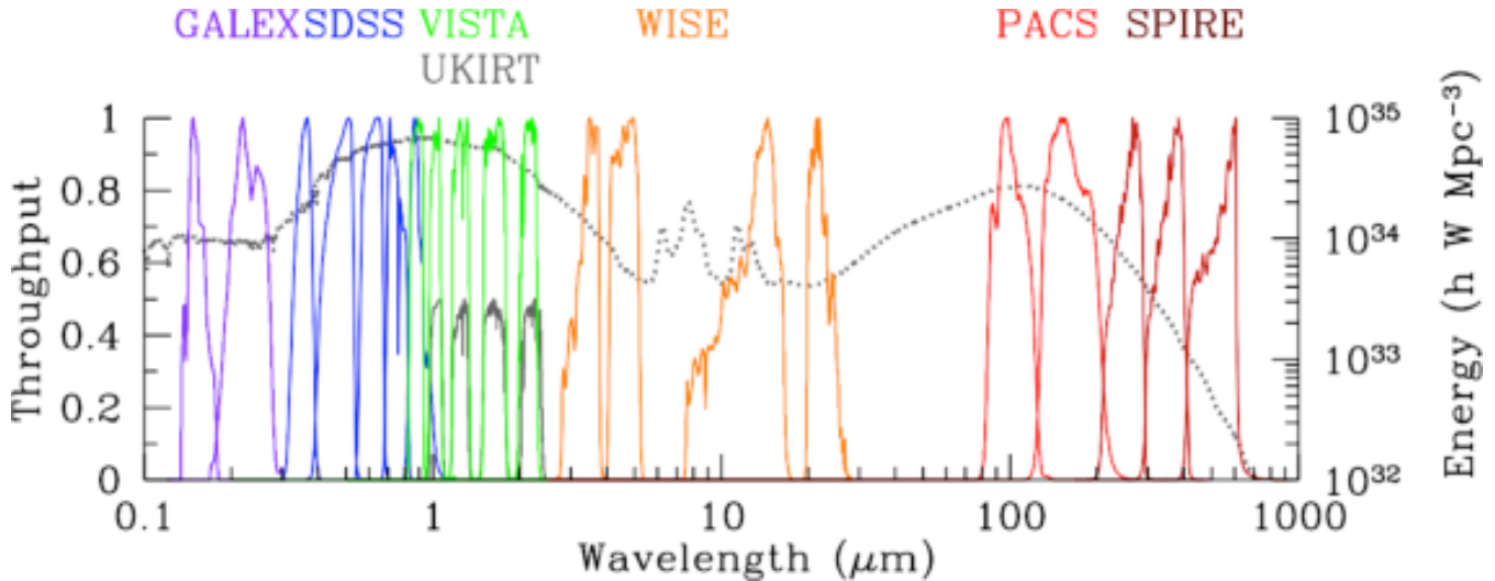
Figure 1. The 21 broad-band combined system throughput curves colour-coded by facility as indicated. Also shown (light grey line) is the recently measured(optical)/predicted(mid and far-IR) cosmic spectral energy distribution derived by Driver et al. (2012). This CSED can be thought of as an energy weighted “canonical” galaxy spectral energy distribution and highlights how the GAMA PDR filter set samples the key energy regime for nearby and low redshift galaxies. Note filters are scaled to a peak throughput of 1 except UKIRT which are scaled to 0.5 for clarity.
