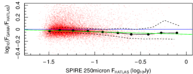
Figure 20. A comparison between the preliminary Herschel-ATLAS 5 \sigma catalogue and the optically motivated catalogue derived here in the SPIRE 250 \mu m band. It should be noted that the zero-points calibration and entire reduction process have evolved between these catalogues. Note units are in Jansky as is standard in the far-IR.
