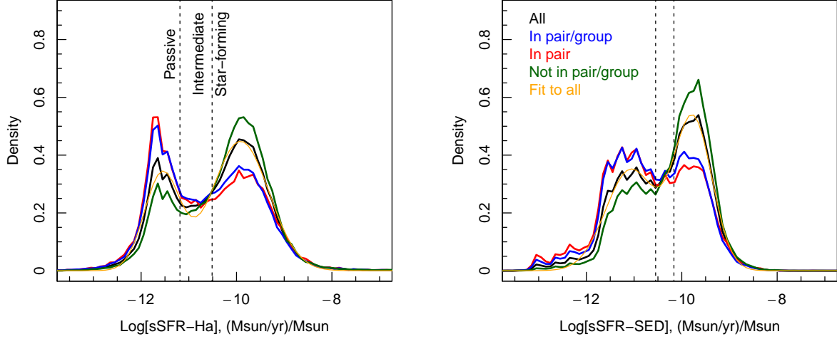
Figure 2. Specific SFR distribution of galaxies in different local environments. Left: for H\alpha derived SFRs and right: for MAGPHYS derived SFRs. Colours show the different environmental classifications defined in Section 2. Orange line displays the double gaussian least squares fit to the distribution of all galaxies (black line). Dashed vertical lines show the lower peak +1\sigma and the upper peak -1\sigma of the orange line. We define galaxies as either passive (lower than left-most dashed vertical line), star-forming (higher than right-most dashed vertical line) or intermediate (between the two dashed vertical lines). We deem the bulk of galaxies in our passive/star-forming selection to be truly passive/star-forming, and ignore all intermediate sources in our subsequent analysis. Considering the different environments, passive galaxies are more likely to be in pair and/or group environments, whereas star-forming galaxies are more likely to be isolated ( i.e. the blue and red passive peak is larger than the full, black, distribution, while the green SF peak is larger than the full, black, distribution).
