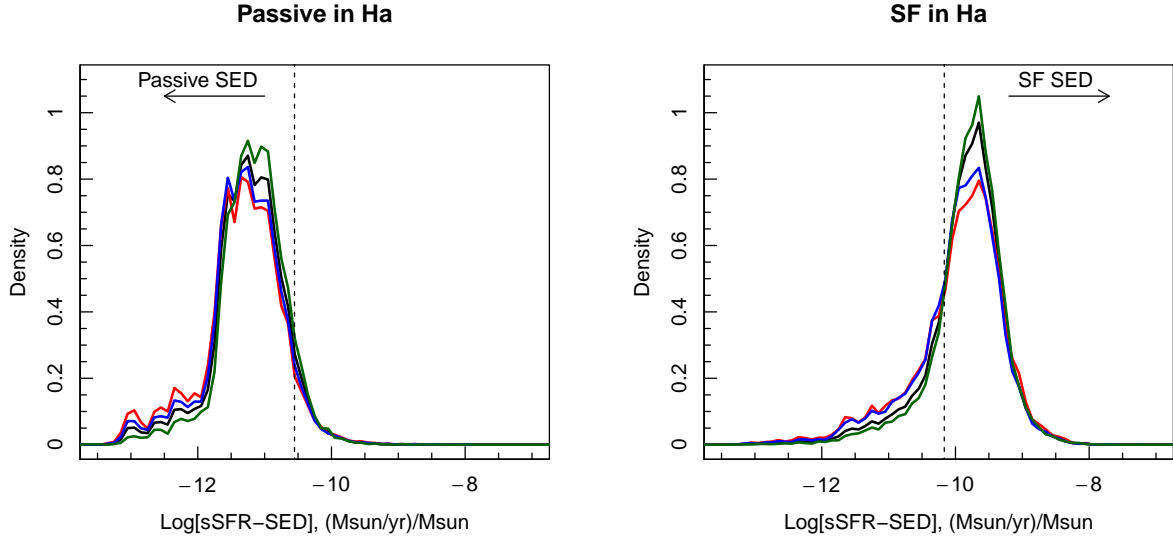
Figure 3. The distribution of MAGPHYS sSFRs, split by sources selected as either passive (left) or star-forming (right) by their H\alpha derived SFRs (left panel of Figure 2). Vertical lines show the passive/intermediate/star-forming split of the right panel of Figure 2. Clearly some sources defined as passive in H\alpha are not when using MAGPHYS and vice versa. As such, we define an additional sample which are selected as star-forming or passive using both classifications ( i.e. they are selected star-forming/passive in both H\alpha and MAGPHYS).
