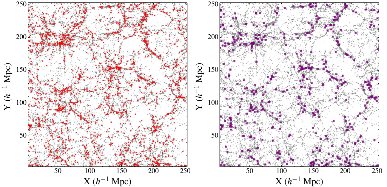
Figure 12. Left panel: distribution of galaxies that have undergone a major merger at any point during their evolutionary histories (red points), taken from the Millennium Simulation. Right panel: the distribution of galaxies that have undergone major mergers in the past 5 Gyr only (purple points). In both plots, all galaxies in a 20 h^{-1} Mpc thick slice of the Millennium simulation at z = 0 are shown as grey points. These grey points are common to both panels. The slice measures 250 h^{-1} Mpc \times 250 h^{-1} Mpc. The plotted galaxies have stellar mass > 5 \times 10^9 M_{\odot} . Galaxies with major mergers in the past 5 Gyr typically avoid the void regions.
