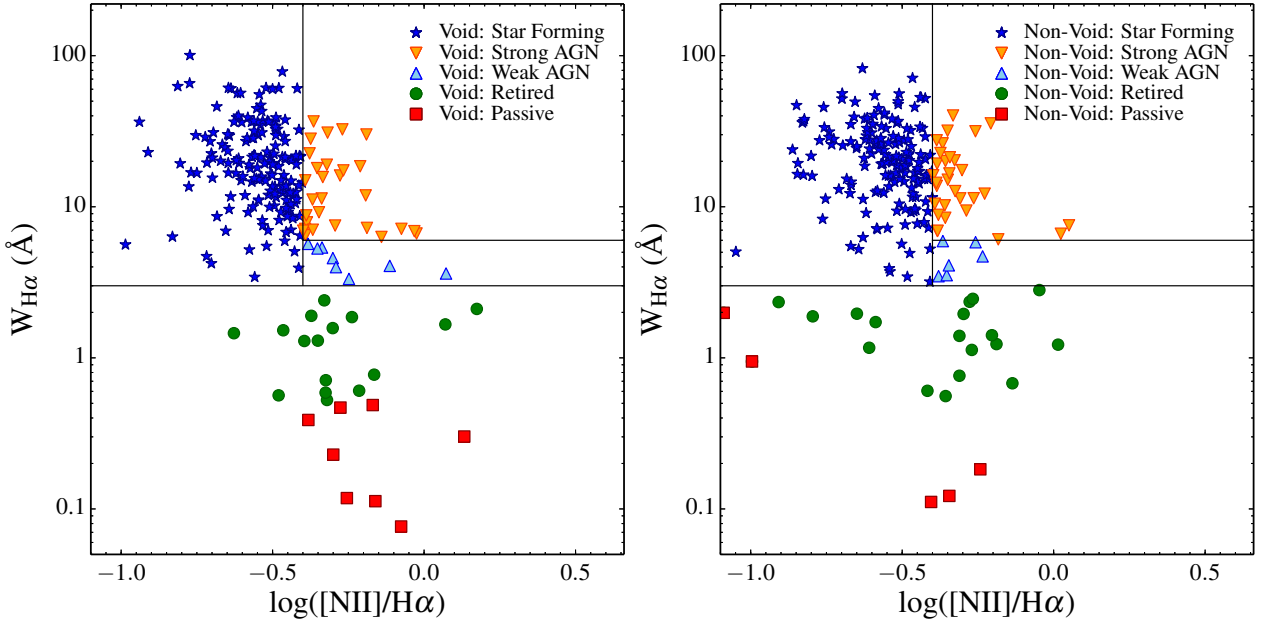
Figure 5. Left-hand panel: W_{H\alpha} vs. [\text{NII}]/H\alpha (WHAN) diagram (Cid Fernandes et al. 2011) for GAMA void galaxies. While the majority of void galaxies are star forming or host AGN, a number of passive/retired galaxies are seen. Right-hand panel: the WHAN diagram for a mass-matched randomly-drawn non-void comparison sample.
