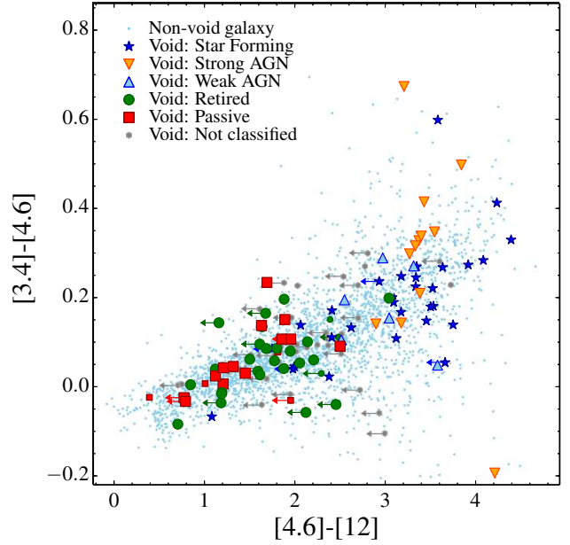
Figure 8. WISE [4.6] - [12] vs. [3.4] - [4.6] ( [W2-W3] vs. [W1-W2] ) colour-colour diagram for void and non-void comparison galaxies with masses > 5 \times 10^9 M_{\odot} and passive optical colours (u-r) > 1.9 . The smaller versions of the symbols have an equivalent width vs. equivalent width error ratio < 3 . The non-void galaxy population occupying the same region of the CMD is also plotted for comparison (blue dots). A range of [4.6] - [12] colours is seen for both the void and comparison galaxy populations, consistent with a range of recent star formation activity.
