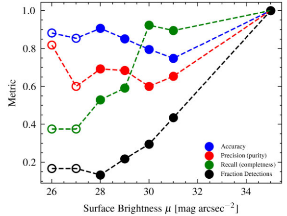
Figure 10. Accuracy (blue), precision (red), and recall (green) obtained for the test sample as a function of the images’ surface brightness \mu_{\text{lim}} . The fraction of tidal detections in the input catalogue is shown in black. The bins at \mu_{\text{lim}} = 26, 27 \text{ mag arcsec}^{-2} are plotted as empty circles to highlight the fact that they are not part of the original sample from M22; the labels used for training and testing are the ones for their corresponding images at \mu = 28 \text{ mag arcsec}^{-2} .
