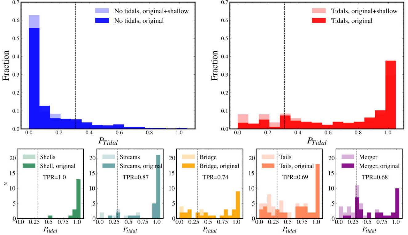
Figure 4. Upper panels: Output probability distribution of the model for tidal detection, P_{Tidal} , for the test sample divided into non-tidal visual classifications (left-hand panel, blue) and tidal visual classifications (right-hand panel, red). Darker colours represent the original sample, lighter colours the shallow sample. Lower panels: P_{Tidal} , for the test sample divided into different categories, as stated in the legend. The dashed line is P_{th} = 0.31 , the threshold used to define an instance as positive or negative. The true positive rate (TPR) of each category for the original + shallow sample is reported in the corresponding panel.
