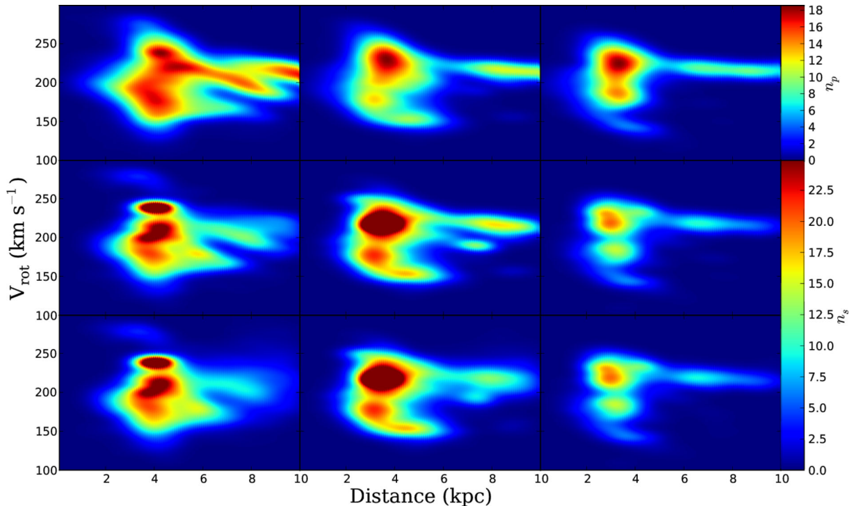
Figure 5. Smoothed linear scale contour plot of heliocentric distance against galactocentric rotation velocity of simulation particles (upper), selected SNAPDRAGONS stars (middle) and selected SNAPDRAGONS stars observed with Gaia error (lower) within a square region of \pm 5 deg around (l, b) = (90, 0) (left), (l, b) = (120, 0) (middle) and (l, b) = (150, 0) (right). For the SNAPDRAGONS stars (middle and lower panels), a limited selection of M_V \leq -1 calculated using V and d_{\text{obs}} and assuming a known extinction, along with \sigma_{v_r}/(v_r \times d_{\text{obs}}) \leq 0.15 is shown to avoid overly dense populations of fainter stars at smaller distances. This is to visualize the data set, and these faint stars contribute to the subsequent analysis. The colour scale shows number density of N -body particles (upper) and SNAPDRAGONS stars (middle and lower) in arbitrary units.
