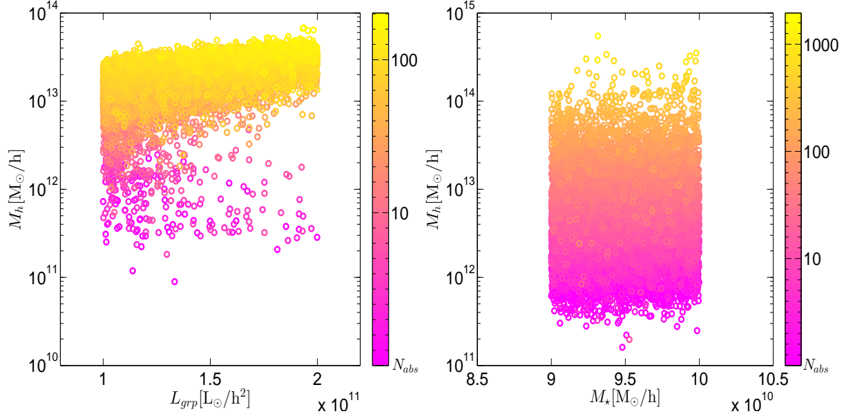
Figure B2. The role of group absolute multiplicity in the mass-observable relations. In the left panel, we plot the halo mass-luminosity relation for all haloes with 10^{11} h^{-2} L_{\odot} < L_{\text{grp}} < 2 \times 10^{11} h^{-2} L_{\odot} , colour-coded by N_{\text{abs}} . The right panel is similar but for the halo mass-central galaxy stellar mass relation of systems with central galaxy stellar masses in the range 9 \times 10^{10} h^{-2} M_{\odot} < M_{\star} < 10^{11} h^{-2} M_{\odot} .
