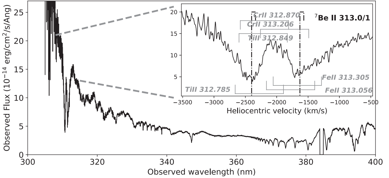
Figure 9 The Day 16 spectrum of ASASSN-19qv in the region 300–400 nm. The inset plot shows the region centred around the \text{Be II } \lambda 313.058 , which shows the expected positions of low ionization transition absorptions of \text{Cr II} , \text{Ti II} , and \text{Fe II} . Velocities are corrected for the heliocentric correction.
