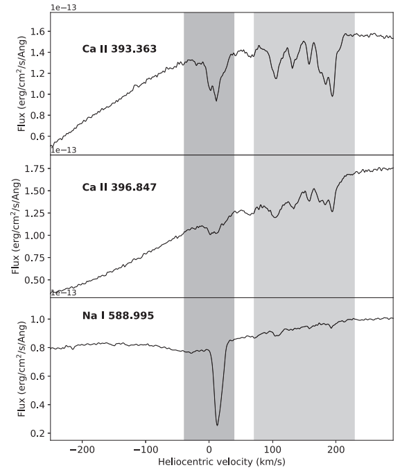
Figure 11. The Day 4 spectrum of ASASSN-20ni centred around the \text{Ca II } \lambda 393.3 (upper panel), the \text{Ca II } \lambda 396.8 lines (middle panel), and around the \text{Na I } \lambda 588.995 \text{ nm} IS line (lower panel). Velocities are corrected for the heliocentric correction. The SMC interstellar \text{Ca II} absorptions are observed at multiple velocity (see the text).
