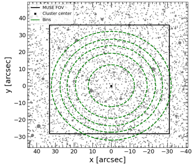
Figure 1. Footprint of the MUSE observations (black box). Green circles represent the bins used for the kinematic analysis, while the black cross is the cluster centre from Dalessandro et al. (2014).
