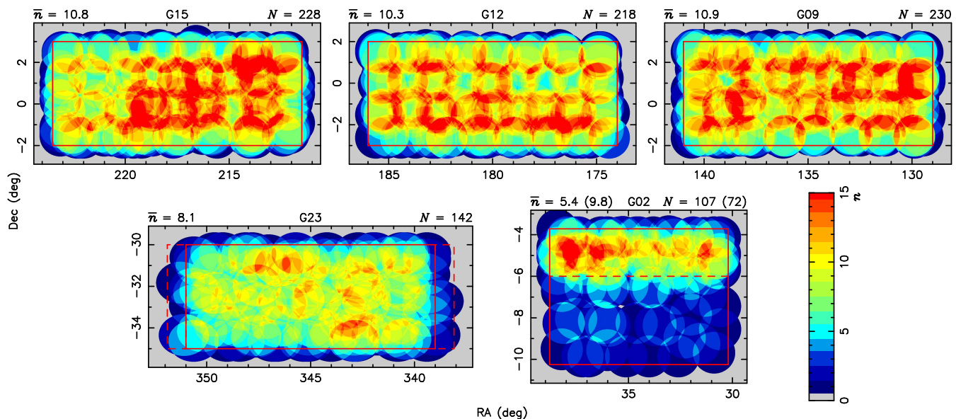
Figure 9. Distribution of observed 2dF/AAOmega fields (assumed to be circles of 1 deg radius) in the GAMA II survey regions. The nominal survey regions are shown as red rectangles. The dashed red lines in G23 indicate the original, slightly more extended region, while the dashed line in G02 shows the lower declination limit of the high-priority sub-region (cf. Table 1). The colour scale indicates the number of fields, n , covering a given position. In each panel, the average value of n within the nominal survey region, \bar{n} , is indicated at the top left, while the total number of fields in each region, N , is indicated at the top right. The numbers in parentheses in the G02 panel refer to the high-priority sub-region.
