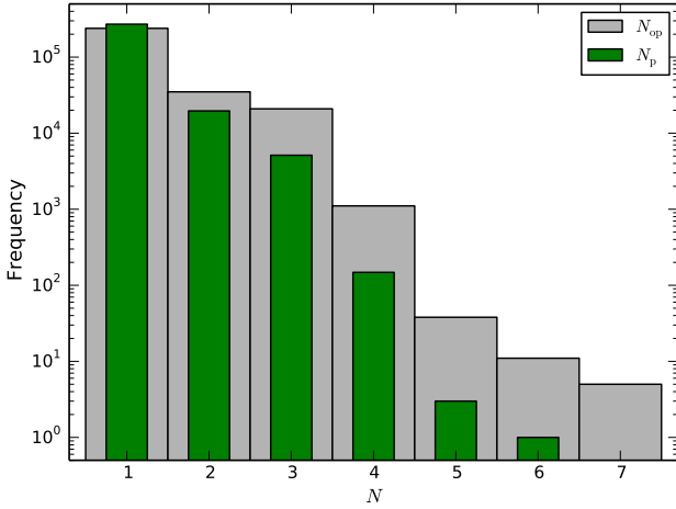
Figure 4. The grey histogram shows the distribution of the number of offered opinions per spectrum, N_{op} , for all GAMA II spectra of main survey targets. The green histogram shows the distribution of the number of possibilities per spectrum, N_p (see text for details).
