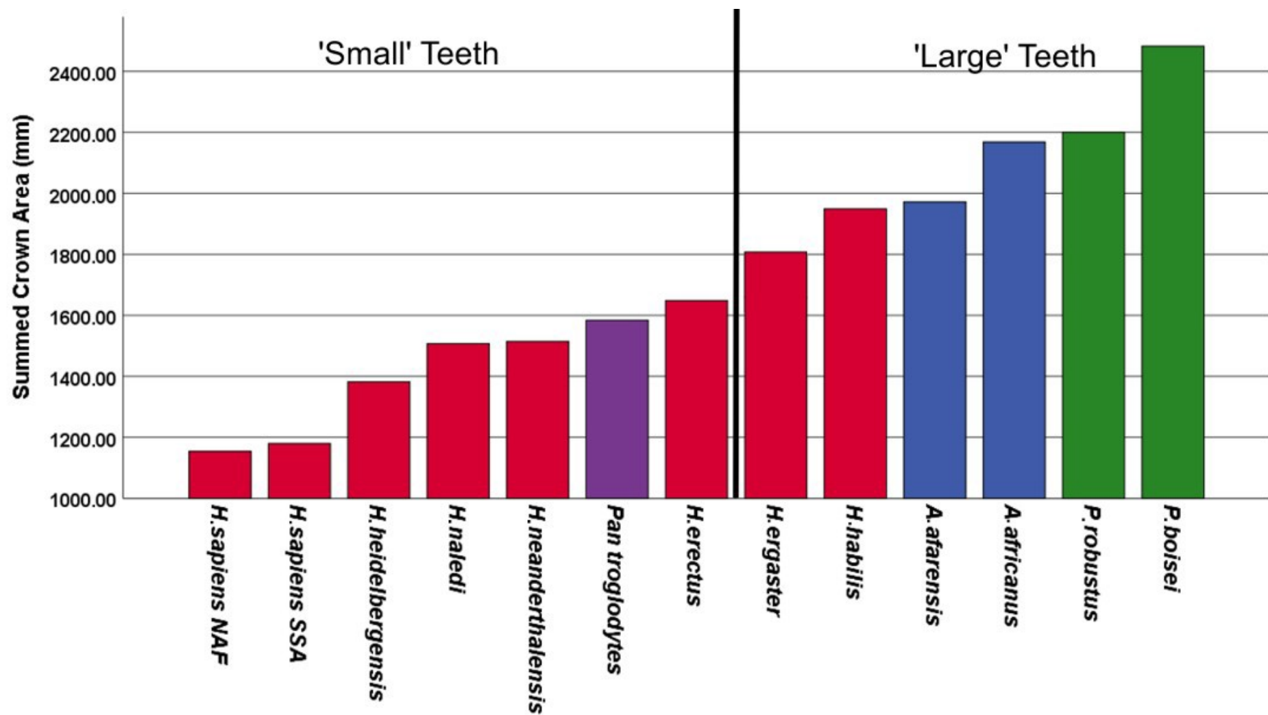
SI FIGURE S2 Bar graph of summed crown areas from unscaled odontometric measurements [(MD x BL) x 16 total maxillary and mandibular teeth)] for all samples to illustrate dichotomy between 'large'- (1813-2483 total mm 2 ) and 'small'-toothed (1154-1638 mm 2 ) species responsible for influencing the UPGMA clusters in SI Figure S1. Color-coding generally matches species in Figures 1-3. See SI S1 and main text for details.
