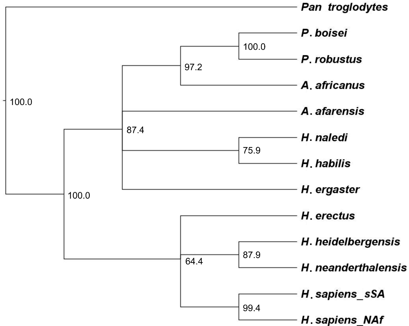
SI FIGURE S8 Bayesian inference cladogram from basic relaxed-clock analysis based on gap-weighted, DM-scaled data under an MKv model of H. naledi and the 12 comparative samples, with clade credibility values for internal nodes included. See main text for details.
