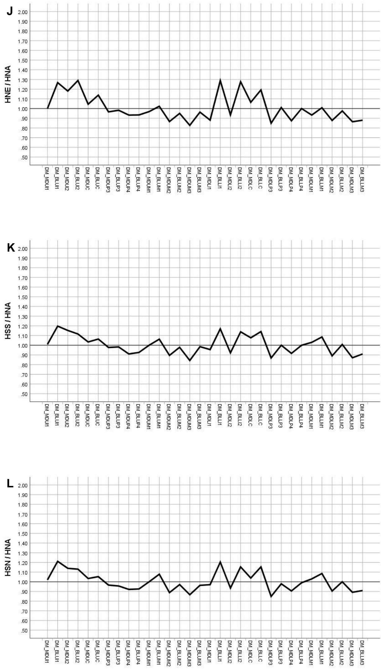
SI FIGURE S9 Line plots of quotients between the dividends A) PAN, B) PBO, C) PRO, D) AFA, E) AFR, F) HHA, G) HEG, H) HER, I) HHE, J) HNE, K) HSS, L) HSN and the divisor HNA for the DM-scaled data, to visualize key characters in H. naledi relative to each comparative sample. Note closest similarity in F, between H. habilis and H. naledi .
