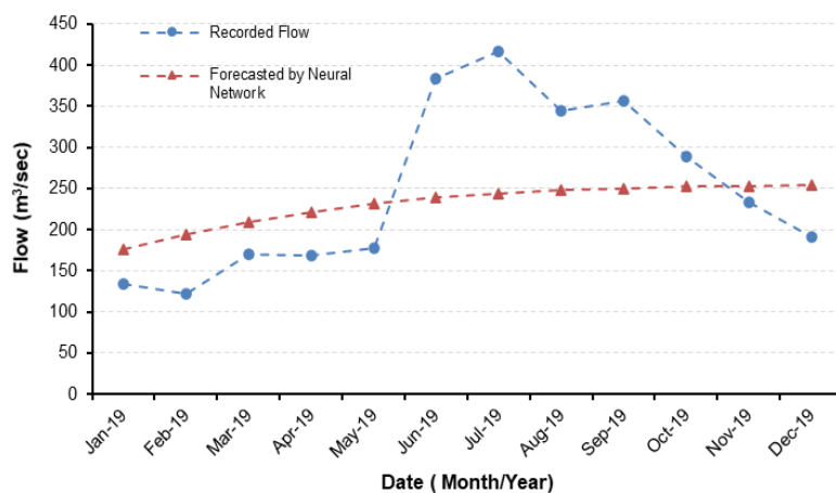
Figure 9: Recorded vs. Forecasted (by ANN) monthly stream flow during 2019.
