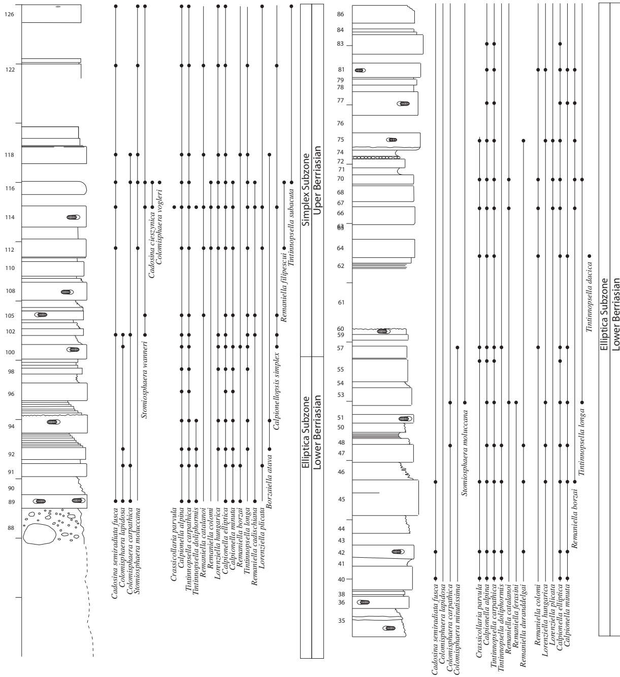
Fig. 6. Hillside upper profile at Tré Maroua (beds 35–126), with calpionellid and calcareous dinocyst ranges, and sample points. Lithologies are as shown in Figure 5. Scale has 1-metre gradations.
