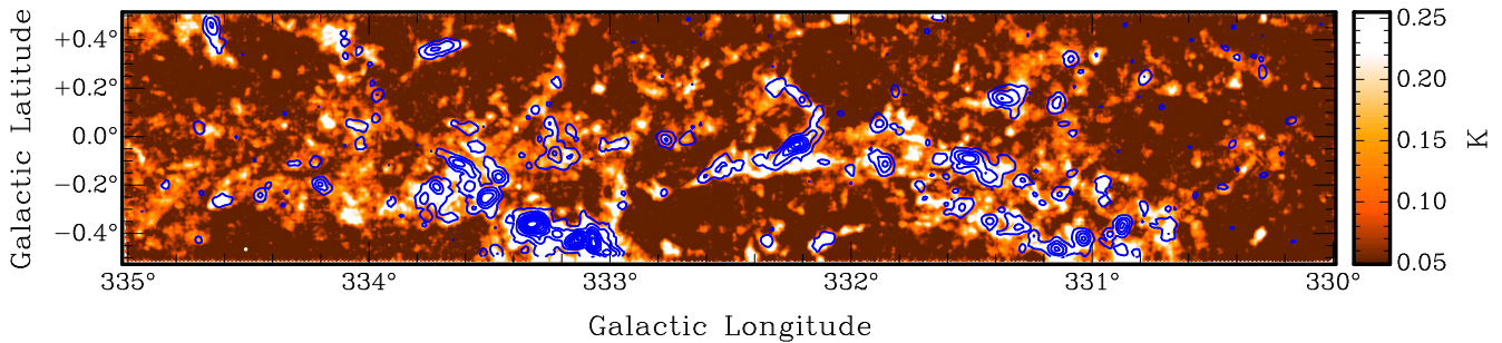
Figure 4: Auto-correlated CS (1–0) peak-intensity map overlaid with HOPS NH 3 (1,1) peak-signal-to-noise contours. Contour levels are 8, 18, ...88 per cent of 11.13 K in units of main-beam temperature. The white circle seen at G334.5–0.45 is the size of the beam.
