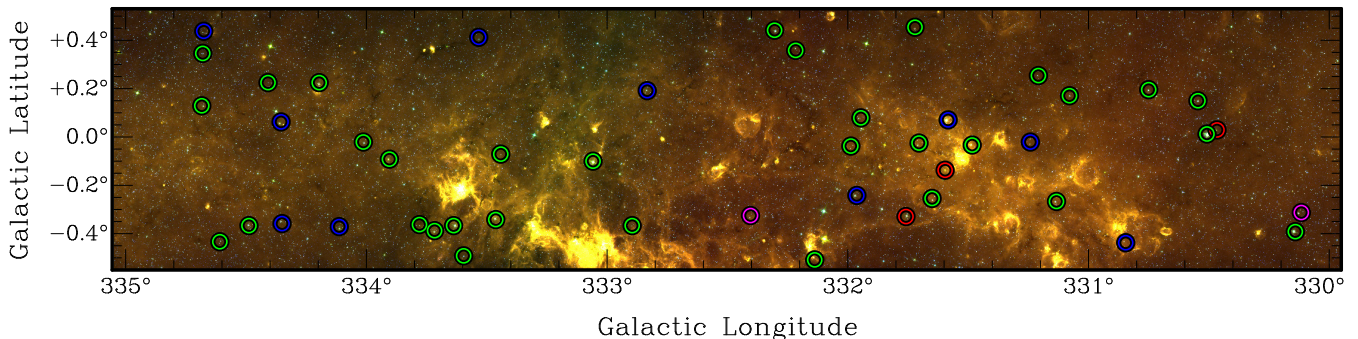
Figure 8: Spitzer GLIMPSE 3-colour (RGB = 3.6, 5.8 and 8.0 \mu\text{m} ) image with MALT-45 positions of detected SiO (1-0) v = 1, 2, 3 masers (circle symbols). The circles have been colour-coded by the vibrational modes within each region. Red: region containing v = 1, 2, 3 maser emission; green: v = 1, 2 ; blue: v = 1 ; magenta: v = 2 .
