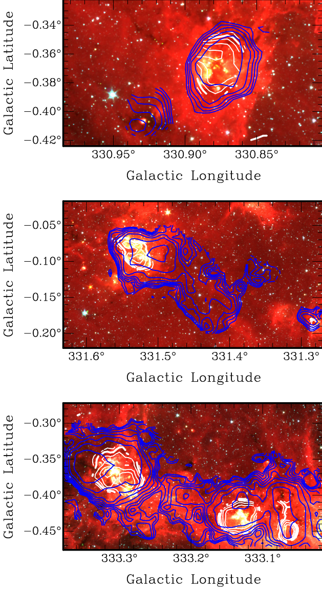
Figure 11. Examples of significant C^{34}S/CS ratios within CS/NH_3 clumps. Spitzer GLIMPSE 3-colour (RGB = 3.6, 4.5 and 8.0\mu m ) image with contours of I(C^{34}S)/I(CS) (white) and contours of I(CS)/I(NH_3) (blue). I(C^{34}S)/I(CS) contour levels are 0.08, 0.10, ..., 0.16, and I(CS)/I(NH_3) contour levels are 0.3, 0.5, ..., 1.9. Note that contour levels for I(CS)/I(NH_3) move from large to small, outside-in. The lowest CS/NH_3 and highest C^{34}S/CS ratios appear to be slightly offset. High C^{34}S/CS ratios appear to occur with bright infrared emission; this is likely due to C^{34}S is only detectable where the overall CS abundance is enhanced in hotter, shocked regions where these molecules have been released into the gas phase.
