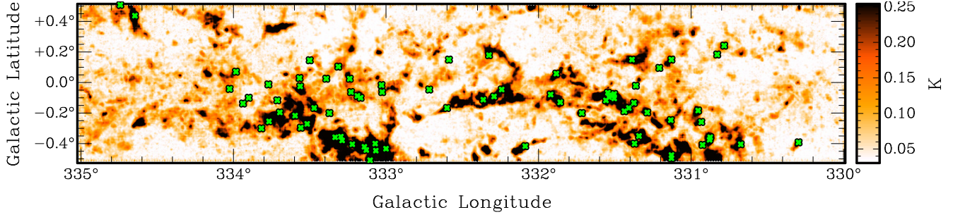
Figure 2: Auto-correlated CS (1–0) peak-intensity map overlaid with positions of detected class I CH 3 OH masers (green cross symbols). A main-beam temperature of 0.1 K represents a 5\sigma peak of emission; note that the RMS of this image is less than that stated in Table 1 (20 mK vs. 34 mK), because this image has been produced by binning channels into groups of 10.
