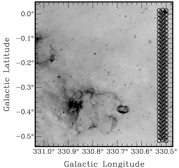
Figure 1. GLIMPSE 8.0 \mu m emission overlaid with part of a MALT-45 mosaic. Each circle represents the primary beam of the ATCA at 49.2 GHz, and is a pointing of the mosaic. Every quarter-square-degree region mapped by MALT-45 is built up of pointing “rows” seen here. These five rows represent the start of the Galactic latitude scans for the G330.5–0.5 region. A similar mosaic is made for each region in Galactic longitude. When both Galactic latitude and longitude mosaics are combined, a fully Nyquist sampled map is obtained. Rows are classified as either “long” or “short”; in this figure, the three long rows have two short rows interleaved.
