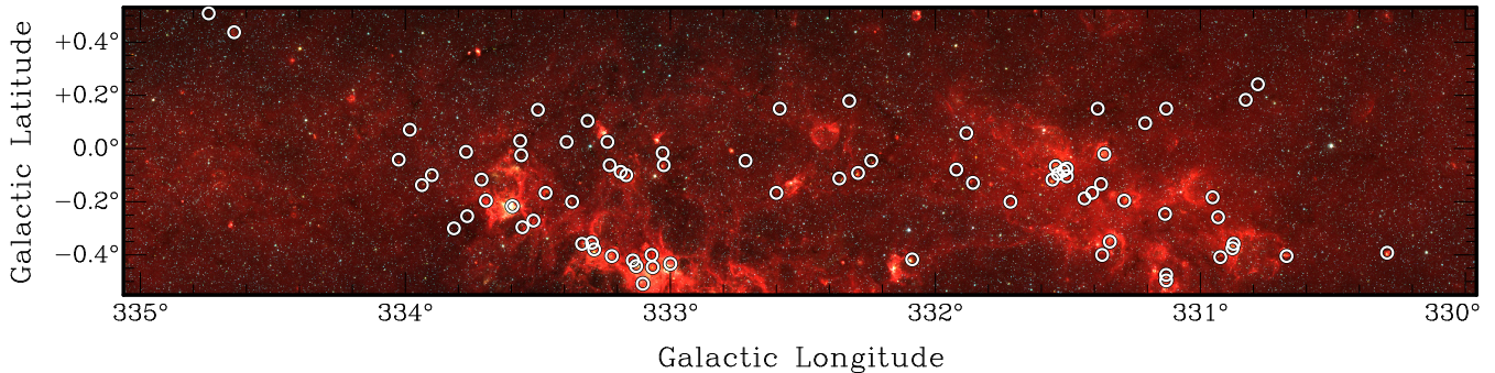
Figure 6: Spitzer GLIMPSE 3-colour (RGB = 3.6, 4.5 and 8.0 \mu\text{m} ) image with MALT-45 positions of class I CH 3 OH masers (circle symbols).
