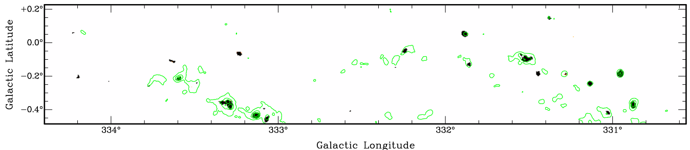
Figure 7: Auto-correlated map of SiO (1-0) v = 0 , overlaid with CS (1-0) thermal emission contours. This image shows SiO emission at and above 0.04 K ( \sim 1.5\sigma ). Contour levels are 14, 34, ...74 per cent of 2.62 K.
