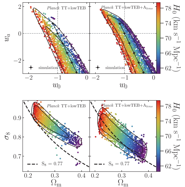
Figure 2. Top: The 1\sigma and 2\sigma constraints in the w_0 – w_a parameter space using Planck TT + lowTEB data, where A_{\text{lens}} has been fixed at unity (left column) or left to vary (right column). The black points show the locations of the simulated cosmologies and the error bars on the points show the size of the region used to generate the rest of the cosmological parameters. The dashed lines cross at the cosmological constant. Bottom: The same as above except for \Omega_m – \sigma_8 , where the dashed line shows S_8 = 0.77 .
