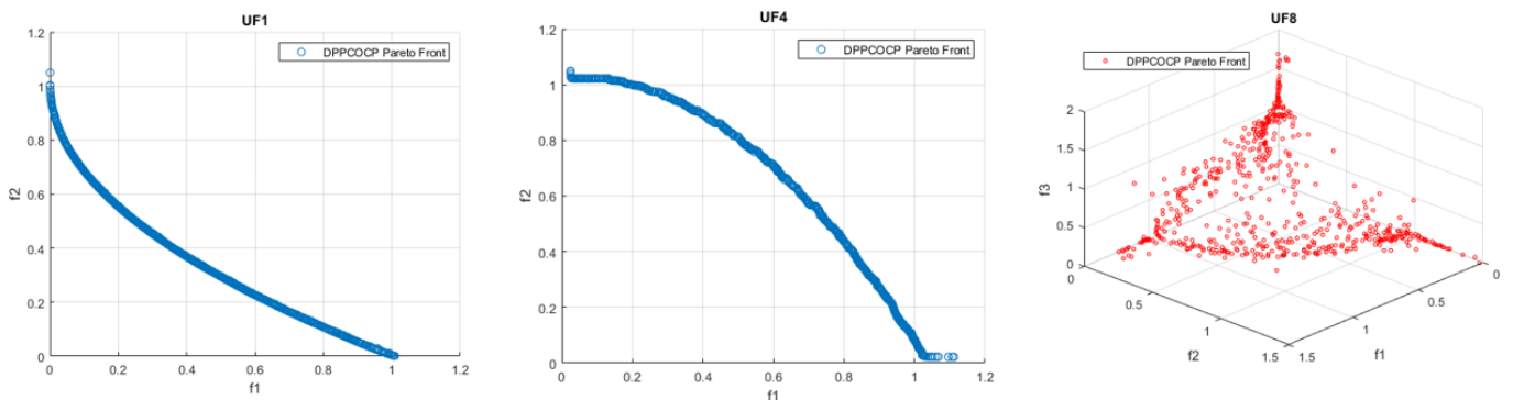
FIGURE 13: Plots of final solutions found by DPPCP algorithm on UF test instances
