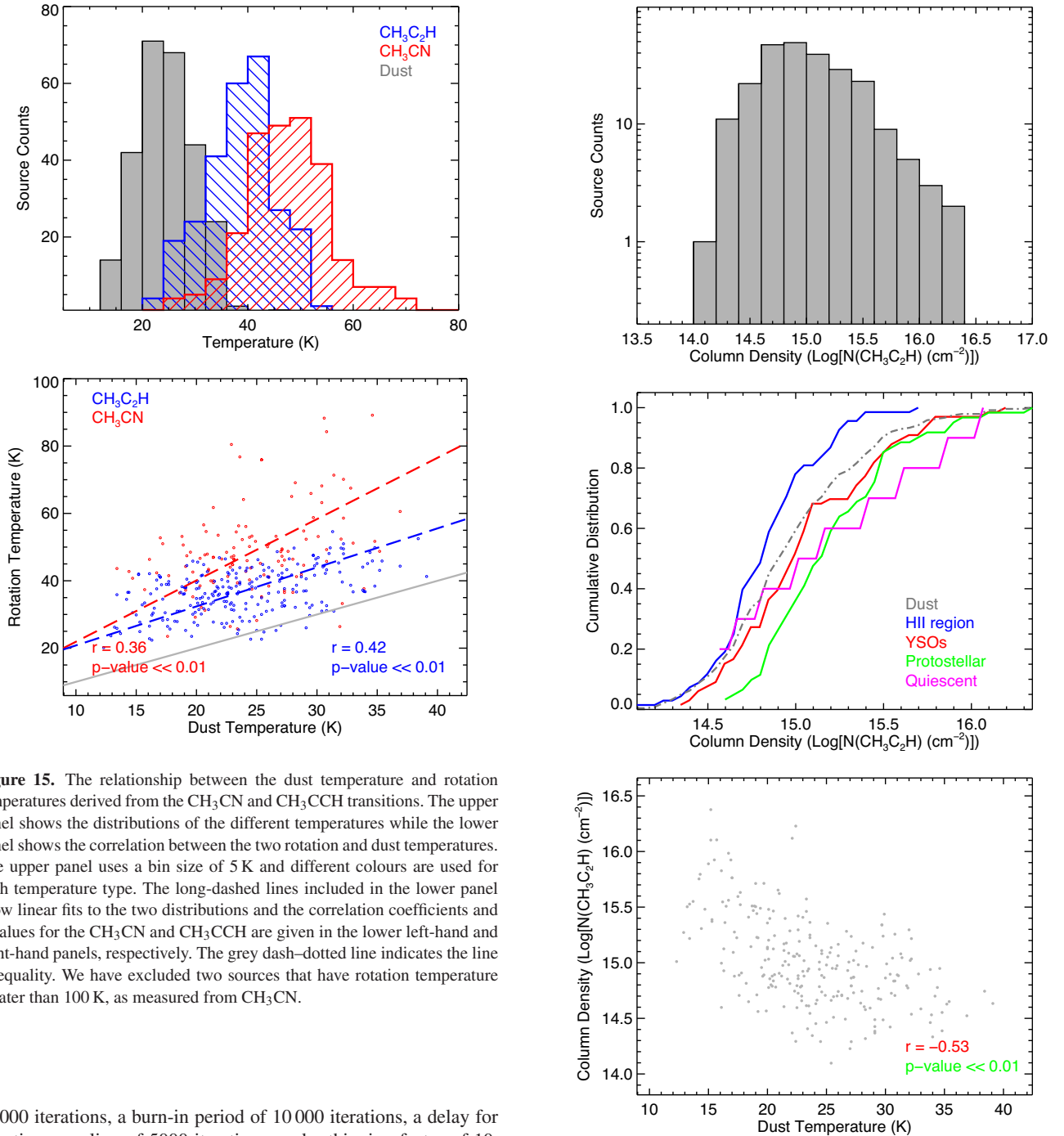
Figure 16. Column density and abundance distributions for \text{CH}_3\text{CCH} . The upper panel shows the column density of the whole sample of 240 detections; the bin size used is 0.2 dex. The middle shows the column density broken down into the four evolutionary stages; the colours of the curves match the colours of the sample names given in the lower right corner of the plot. The lower panel is a scatter plot showing the relation between the fractional abundance of \text{CH}_3\text{CCH} relative to \text{H}_2 and the dust temperature; in the lower right corner we give the Spearman coefficient and associated p -value.
